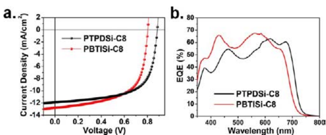
Figure 12. (a) Illuminated J - V characteristics and (b) external quantum efficiency spectra of optimized PBTiSi-C8 and PTPDSi-C8-based solar cells.
