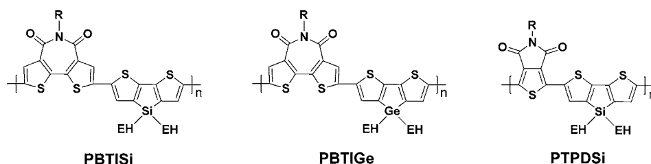
Figure 4. Structures of bithiopheneimide and dithienosilole copolymers ( PBTiSi ) and bithiopheneimide and dithienogermole ( PBTiGe ) copolymers for efficient polymer solar cells. Thieno[3,4- c ]pyrrole-4,6-dione and dithienosilole copolymer ( PTPDSi ) 38c were synthesized for comparison. EH = 2-ethylhexyl.
